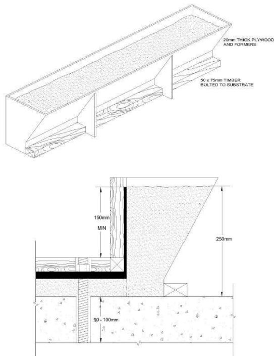
Fig.2 Typical Hopper detail
